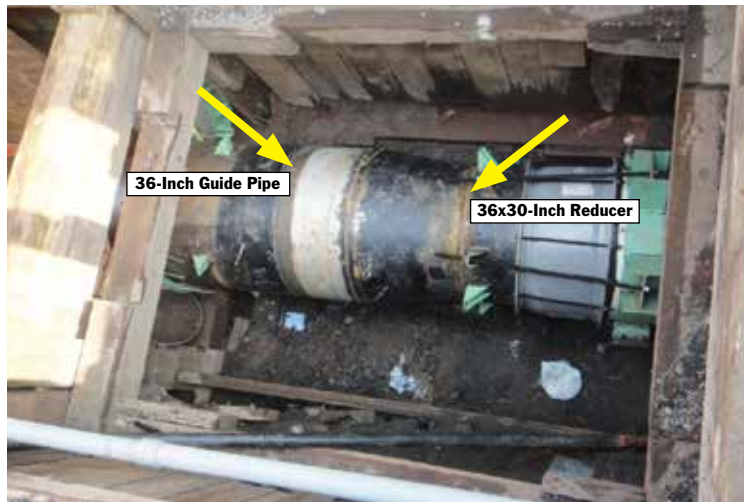
CIP lining through a 36-inch Guide Pipe, two 36x30-inch reducers, and a 30-inch gate valve has never been accomplished anywhere before
