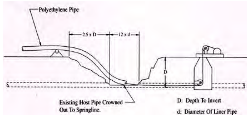
Sample of Common Insertion Pit Configuration for Continuous Pipe Installation (Shows details for HDPE Insertion as reference)
