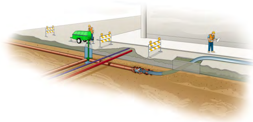
Typical small diameter (6"-12") pneumatic pipe burst utilizing the "manhole exit" method.
